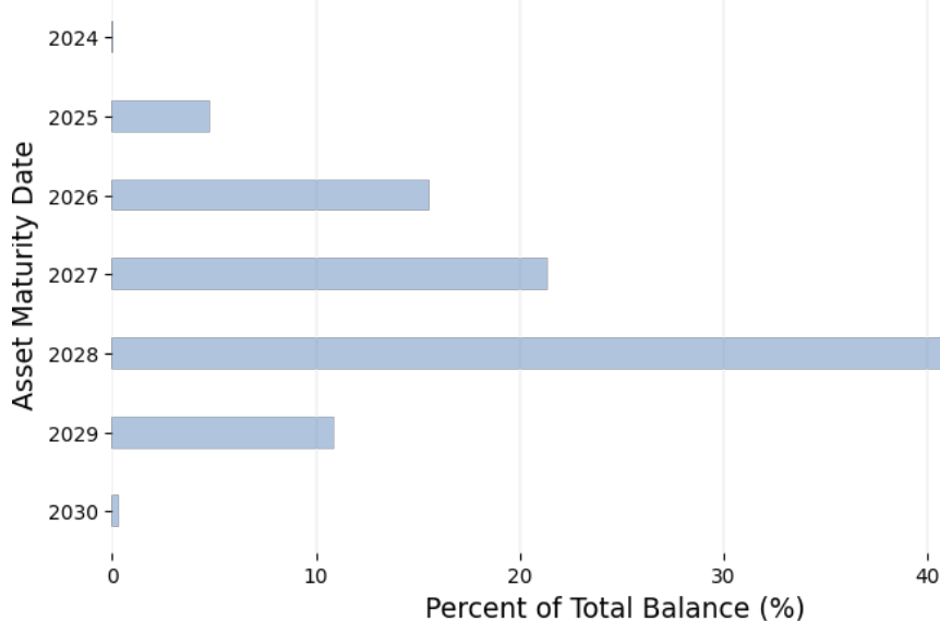
Asset Maturity Distribution
